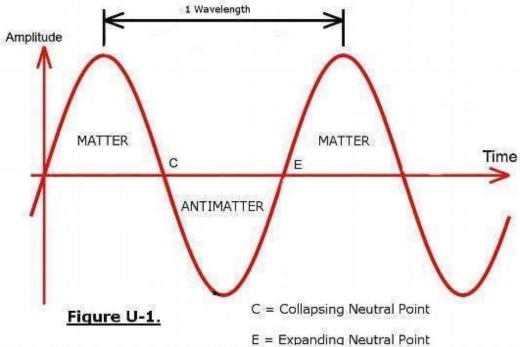
Figure 2. Sine wave of our Blinking Universe.
