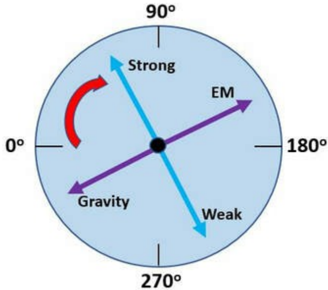
Figure 1. The four fundamental forces are related by phase angle, such that when gravity and the electromagnetic force are near zero (sin 180), then the strong force and weak force are at their largest value. The four fundamental forces are constantly varying.
